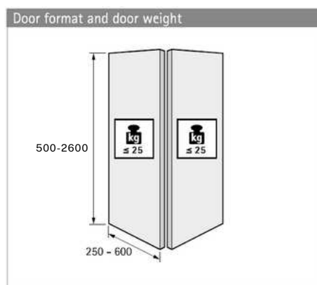
Two part centre hinge
